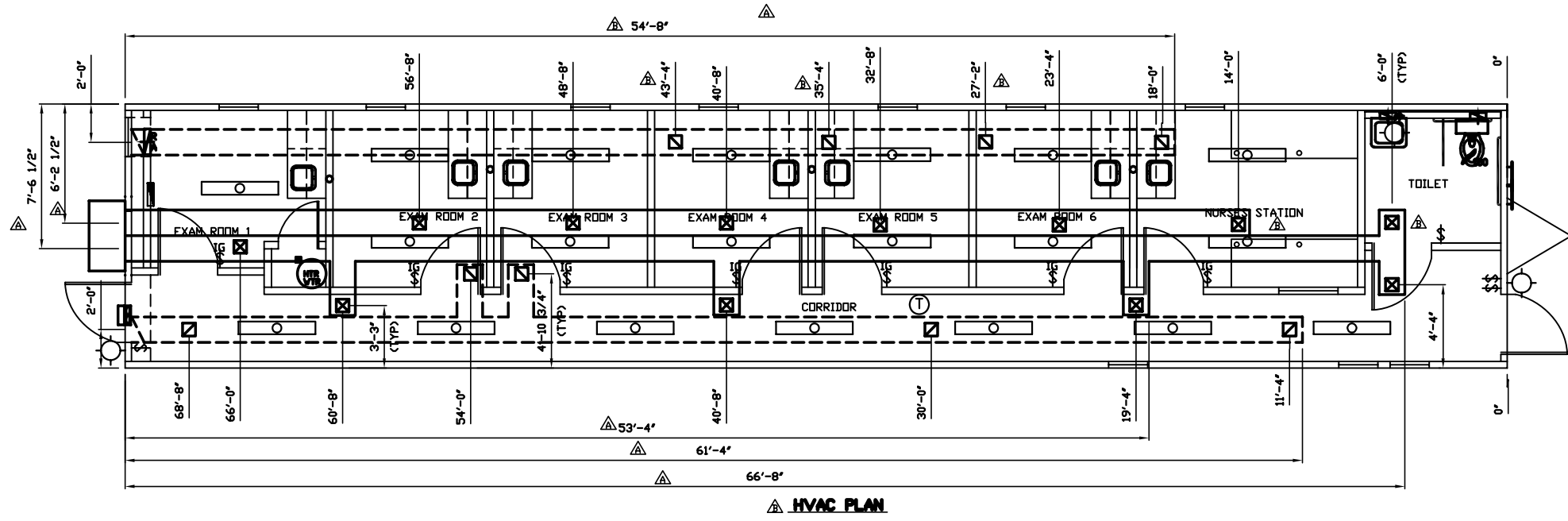
HVAC PLAN
