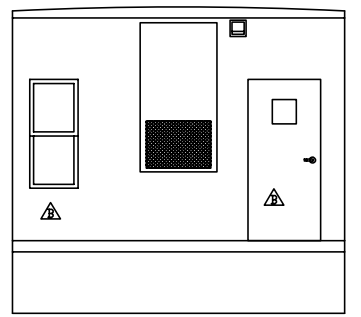
REAR END ELEVATION SCALE: 1/4"=1'-0"
