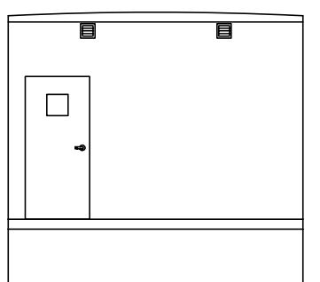
HITCH END ELEVATION SCALE: 1/4"=1'-0"
