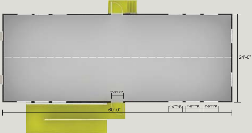
Floor plan
