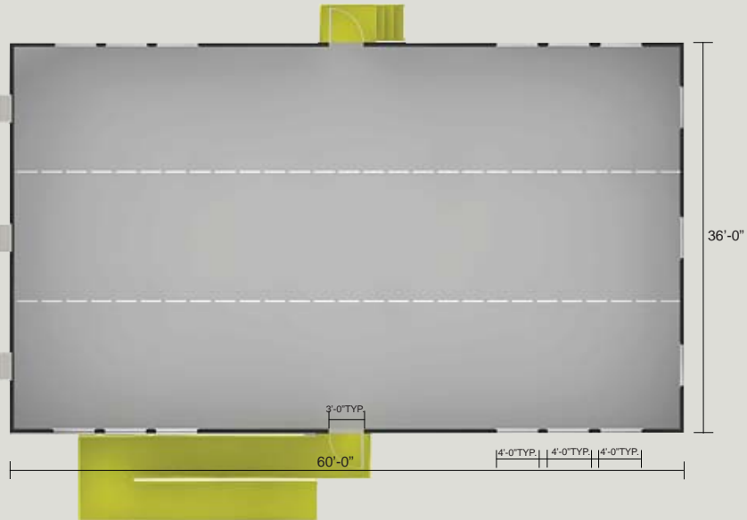
Floor plan
