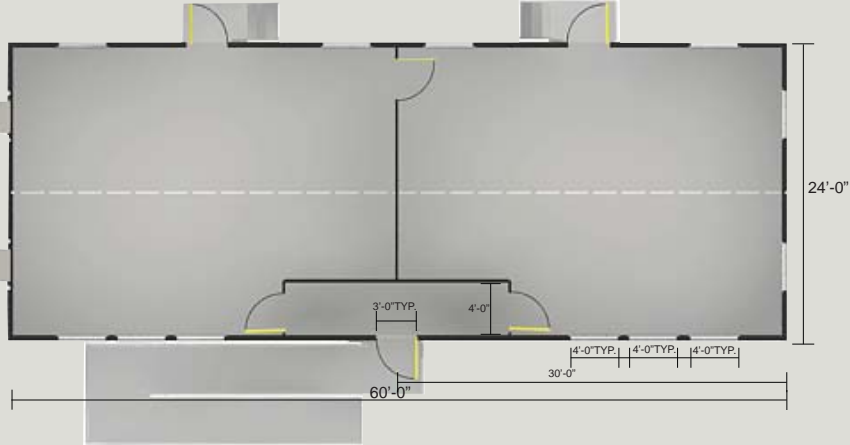
Floor plan
