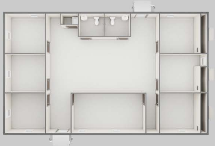
Three Piece BLOCS™ Modular Building with 6 Offices and Conference Room
